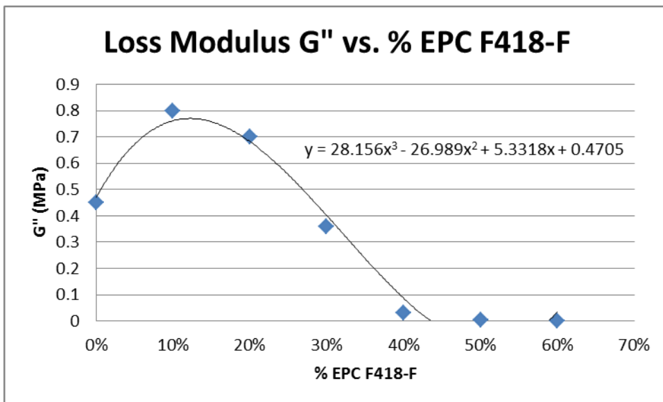
Graph 3: Loss modulus G'' vs. percentage of Silmer EPC F418-F in cycloaliphatic epoxy/anhydride system
