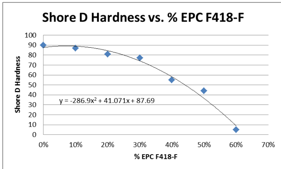
Graph 1: Shore D hardness vs. percentage of Silmer EPC F418-F in cycloaliphatic epoxy/anhydride system
